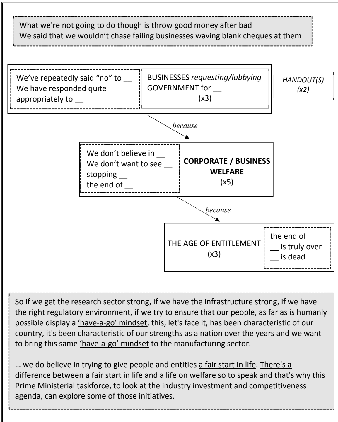
Figure 2: The logic of Mr Abbott’s talk about corporate welfare
